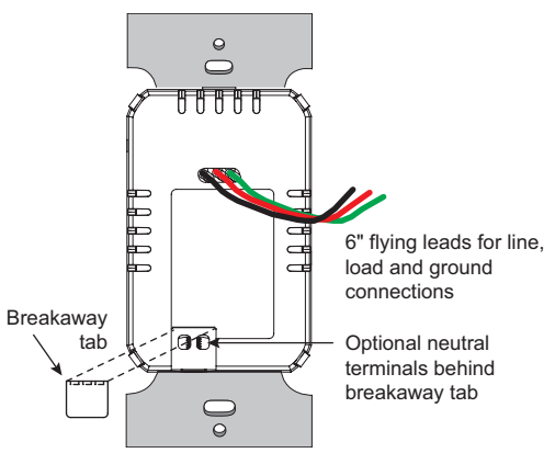
Single-level wiring
