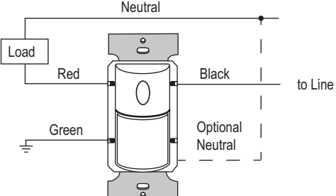
Single-level wiring
