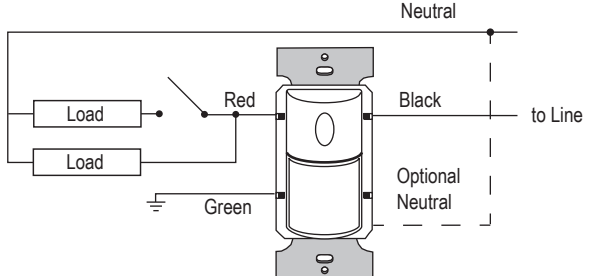
Manual bi-level lighting wiring
