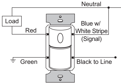
Single-level wiring
