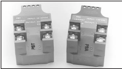
Photo shows DC power block (left) and AC power block (right). DC power blocks have gray housings; AC models are red.
