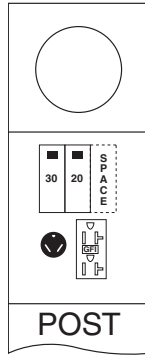
Fig. B M041CP6010, R041CP6010 R32U, 5-20R2GFCI
