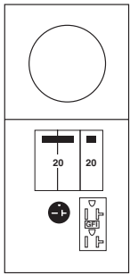
Fig. A M036C010, R036C010 6-20R, 5-20R2GFCI
