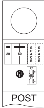
Fig. F M355CP6010, R355CP6010 BR54U, 5-20R2GFCI
