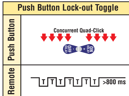
Figure 16. Lockout toggle
