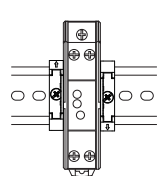
Mounting A (Vertical, standard)
