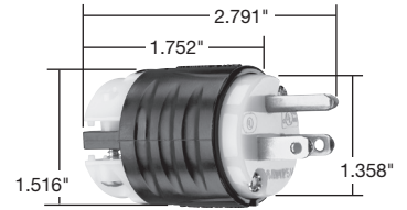
Dimensions for 15 & 20 Amp Plug
