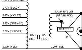
Wiring Diagram 2
