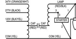
Wiring Diagram 3
