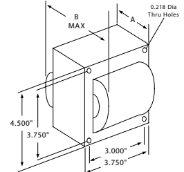
REFERENCE DRAWING 2
