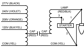
Wiring Diagram 1
