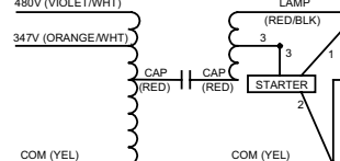
Wiring Diagram 23
