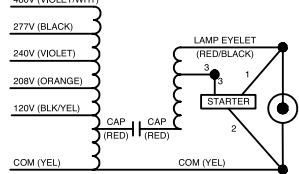
Wiring Diagram 2
