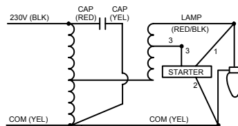
Wiring Diagram 16
