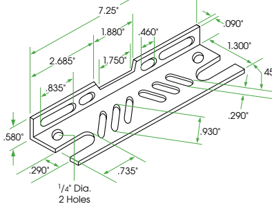
Ref. Drawing MB2
