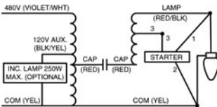
Wiring Diagram 4
