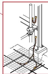
Prefabricated Mesh for Switch Shaft and Operating Handle Grounding
