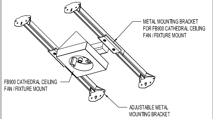
ISOMETRIC ASSEMBLY VIEW
