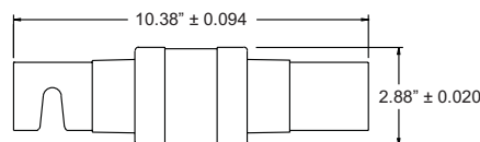
450 to 600A
