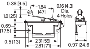
Roller Lever Type
