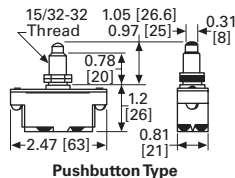
Pushbutton Type
