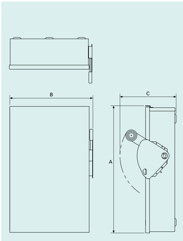
Type 3R solar switch dimensions ❶
