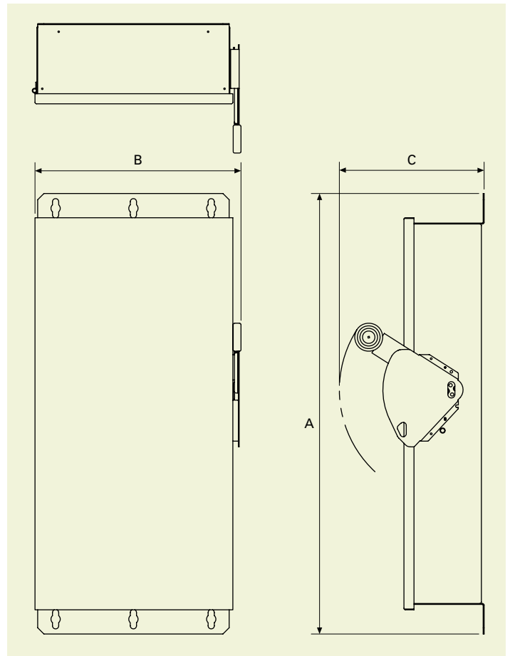
Type 12-3R and 4X solar switch dimensions
