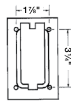
Typical FS mount hole pattern
