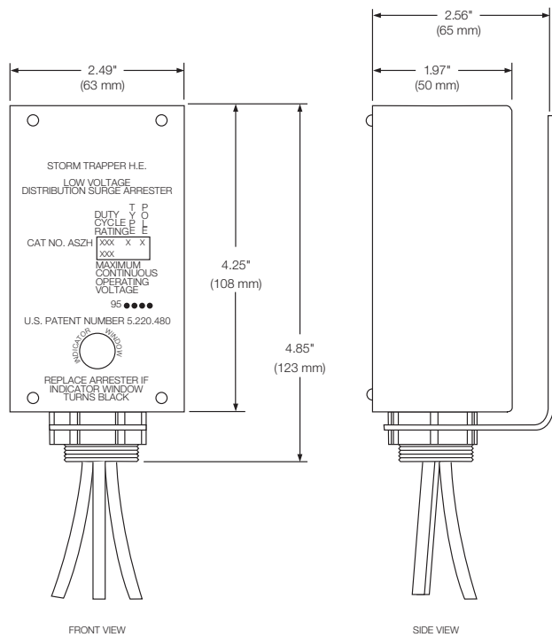
Figure 1. Metal enclosed VariSTAR Storm Trapper high energy MOV arrester with optional mounting bracket.
