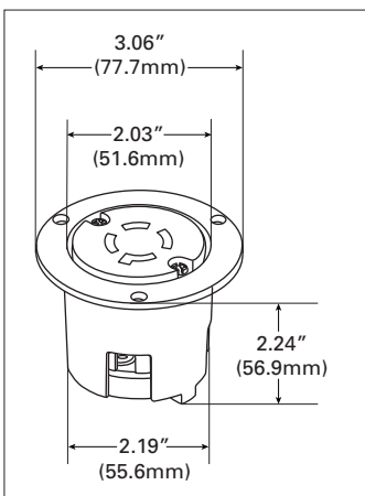
Figure 5. AHCL1420FO
