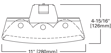
4' or 8', 3 LAMPS
