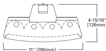
4' or 8', 4 LAMPS
