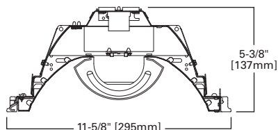
1' x 4' RECESSED
