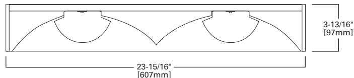
2' x 2' SURFACE
