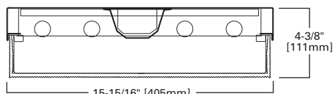
4', 4 LAMP (A)
