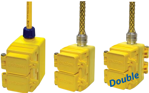
6212NFS Box with 1610-PWDX "pendant non-metallic" style 6234WFS with 1610-PWDX pendant style Double 1610-PWDX on 6234WFT enclosure
