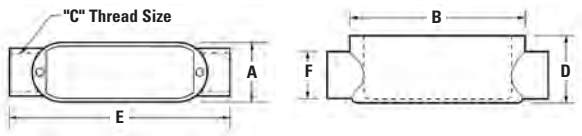
Type C Dimensions—Threaded & Set Screw
